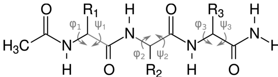
Fig. 2 N-Acetylated tripeptides used for the calculations and experiments, with the main chain dihedral angles ( \phi and \psi ) highlighted.
