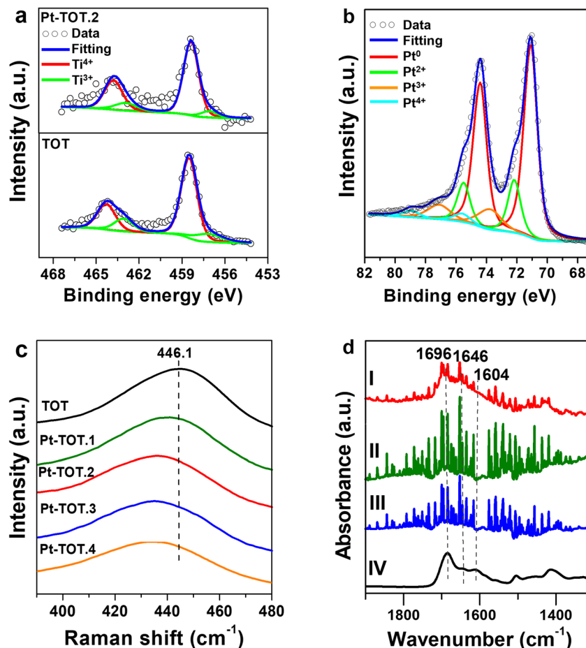
Fig. 4 (a) Ti 2p XPS spectra of TOT and Pt-TOT.2, (b) Pt 4f XPS spectra of Pt-TOT.2, (c) Raman spectra and of TOT and Pt-TOTs in the range from 390 to 480 cm^{-1} , and (d) FT-IR of adsorbed NAD^+ on the surface of (I) Pt-TOT.2, (II) TOT (III) Ti, and (IV) ATR-IR spectrum of the NAD^+ crystal (95%).
