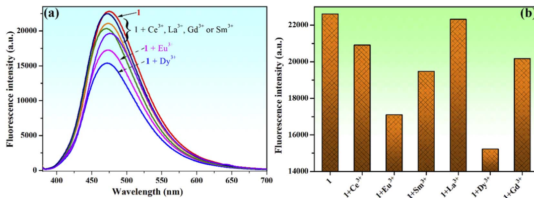
Fig. 10 Change in the fluorescence spectrum (a) and fluorescence intensity (b) of compound 1 ( 10^{-4} M) upon mixing with different rare earth metal ions (2 equivalents of \text{La}^{3+} , \text{Ce}^{3+} , \text{Eu}^{3+} , \text{Dy}^{3+} , \text{Sm}^{3+} and \text{Gd}^{3+} ) in methanol–water (85 : 15, v/v) when \lambda_{\text{ex}} = 365 nm.
