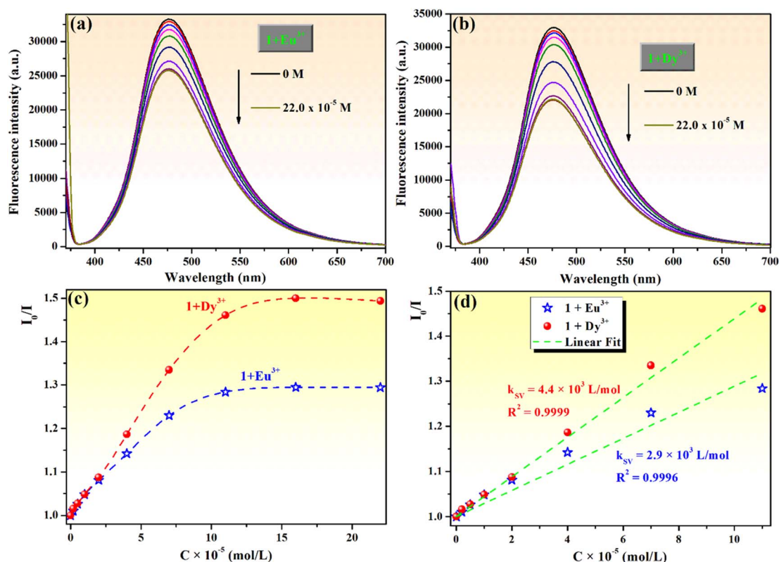
Fig. 11 Fluorescence spectra of compound 1 ( 10^{-4} M) upon addition of different concentrations (0–2.2 equivalents) of (a) \text{Eu}^{3+} and (b) \text{Dy}^{3+} ions. Stern–Volmer plots (c) and linear fit of Stern–Volmer plots in the concentration range of 0– 11 \times 10^{-5} M (d) for the interactions between compound 1 and \text{Eu}^{3+} or \text{Dy}^{3+} ions (at \lambda_{\text{ex}} = 365 nm).
