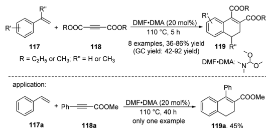
Scheme 34 Synthesis of ADHNs via DMF·DMA-catalyzed cyclic addition of vinylarenes with acetylenedicarboxylate.
