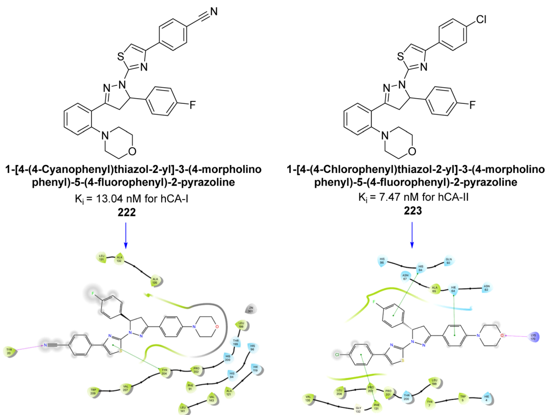
Fig. 80 Chemical structures of compounds 219, 220 and 221; their K_i values against hCA-IX along with docking image of compound 220.
