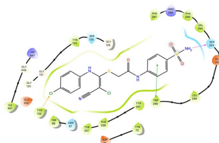
2-[1-(4-Chlorophenylamino)-2,2-dicyanovinylthio]-N-(4-sulfamoylphenyl)acetamide
