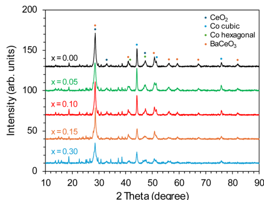
Fig. 3 PXRD patterns of the Co/BaCe 1-x Y x O 3-δ ( x = 0-0.30 ) catalysts after reduction in hydrogen at 600 °C.
