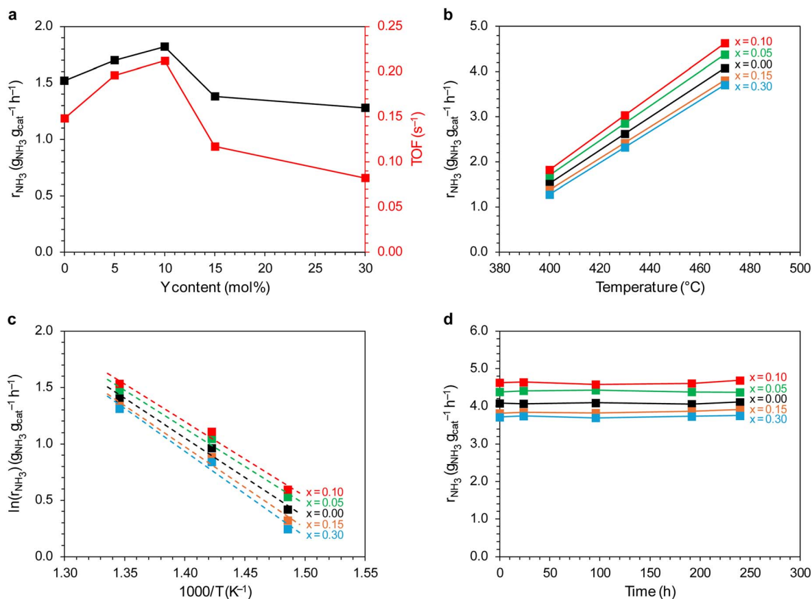
Fig. 13 Evaluation of the catalytic performance of Co/BaCe _{1-x}Y_xO_{3-\delta} ( x = 0-0.30 ) catalysts in the ammonia synthesis reaction. (a) Dependence of the ammonia synthesis rate (400 °C, 6.3 MPa, H_2/N_2 = 3 ) on the yttrium content in the support. (b) Temperature dependence of the ammonia synthesis rate at 6.3 MPa. (c) Arrhenius plots of ammonia synthesis over studied catalysts (6.3 MPa, H_2/N_2 = 3 ). (d) Time-on-stream performance of the studied catalysts (470 °C, 6.3 MPa, H_2/N_2 = 3 ). The catalysts were kept at 600 °C between measurements (240 h in total).
