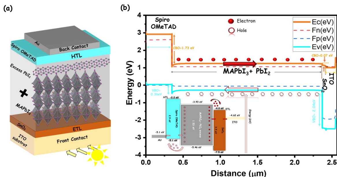
Fig. 1 (a) Schematic of a n-i-p structure for the PSC used in SCAPS simulations: \text{ITO}/\text{SnO}_2/\text{MAPbI}_3/\text{spiro-OMeTAD}/\text{Au} ; (b) energy band diagram for the device. Inset: an energy level diagram of different materials used in the PSC with the values of BC and BV of the ETL and HTL of the selected materials.
