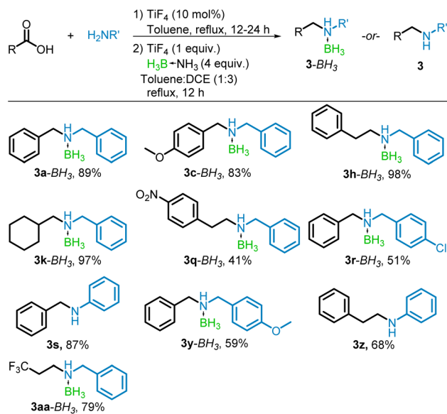
Scheme 5 One pot \text{TiF}_4 -catalyzed reductive amination of acids with \text{BH}_3\text{NH}_3 . Isolated yields shown.
