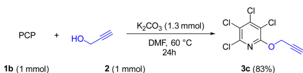
Scheme 5 Site-selective synthesis of 2,3,4,5-tetrachloro-6-(prop-2-yn-1-yloxy)pyridine 3c .
