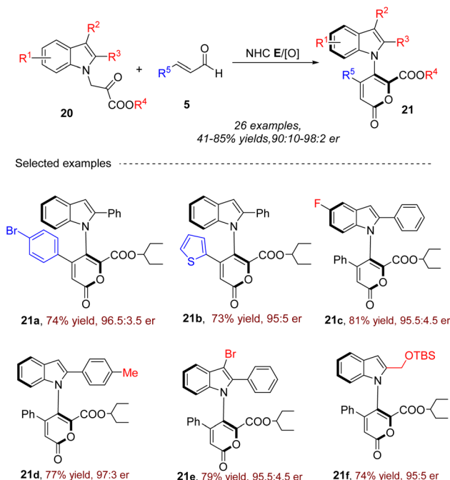
Scheme 9 The synthesis of 5-indo-1-yl pyran-2-ones with an N-C axis from indole-1-pyruvate esters and enals.
