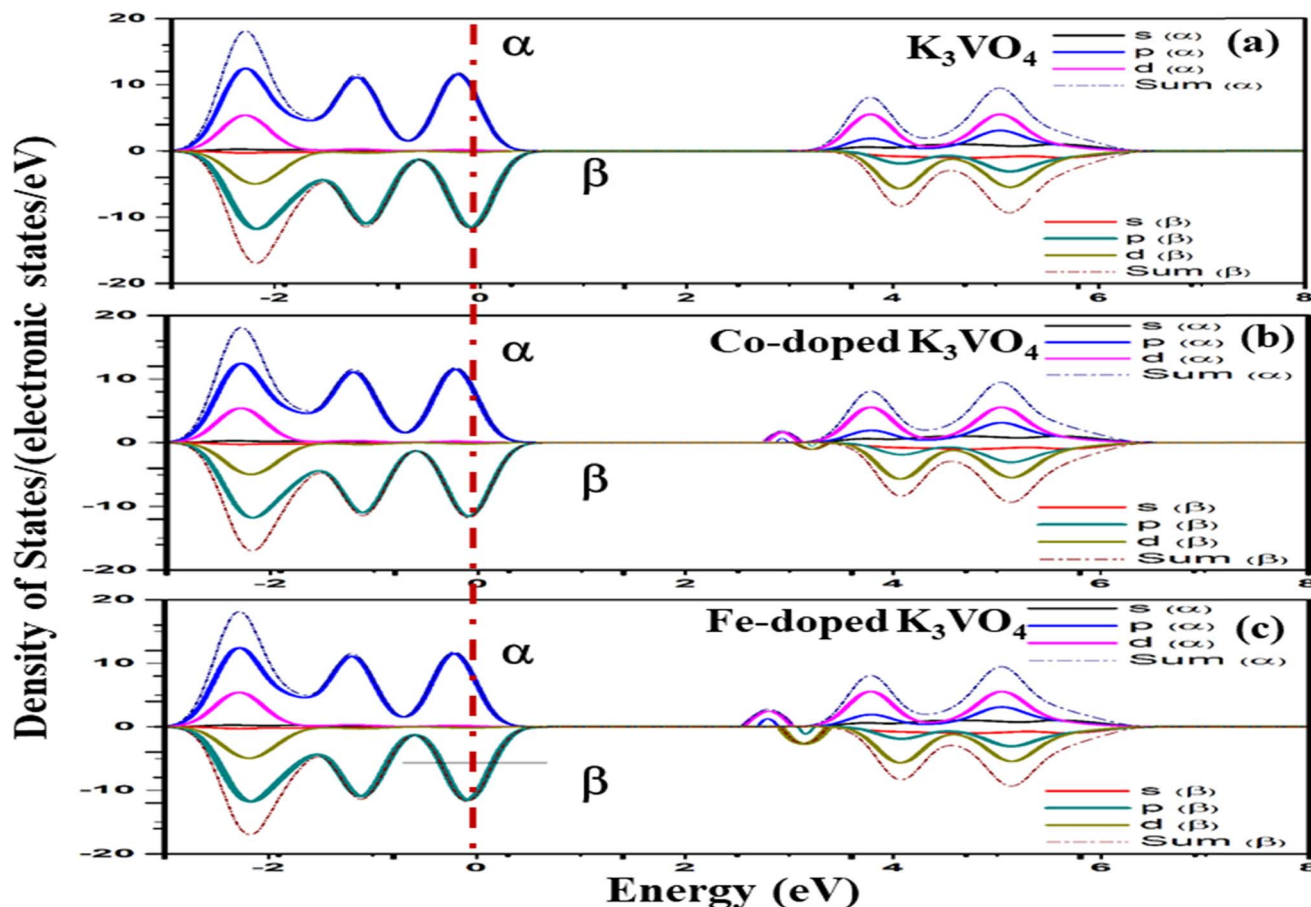
Fig. 14 Spin-up (↑) and spin-down (↓) partial density of states of (a) \text{K}_3\text{VO}_4 , (b) \text{K}_3\text{V}_{(1-0.06)}\text{Co}_{0.06}\text{O}_4 , and (c) \text{K}_3\text{V}_{(1-0.06)}\text{Fe}_{0.06}\text{O}_4 with indicated dashed lines as the Fermi level ( E_F ).
