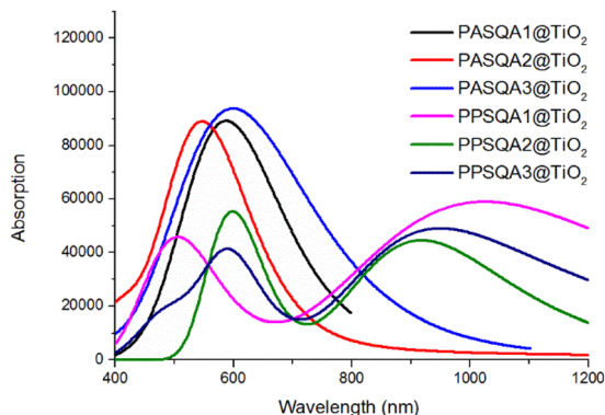
Fig. 7 Absorption spectra in acetonitrile of dyes@TiO 2 at TD-CAM-B3LYP/6-31G(d)/LANL2DZ/SMD level. The spectra are Gaussian broadened with 0.35 eV (half width half maximum).
