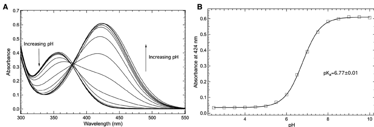
Fig. 2 Room temperature absorbance spectra of the free noncanonical amino acid, 3-nitro-L-tyrosine ( m\text{NO}_2\text{Y} , (A)) as a function of pH in the 300–550 nm region. The ncAA ( 10\ \mu\text{M} ) was dissolved in 50 mM potassium phosphate buffers with pH values ranging from 2.50–10.00. The pH dependence of the absorbance of m\text{NO}_2\text{Y} measured at 424 nm (open squares, (B)) was fit (solid curve) to eqn (1) to yield a pK_a of 6.77 \pm 0.01 of the 3-nitrophenolic hydrogen of m\text{NO}_2\text{Y} .
