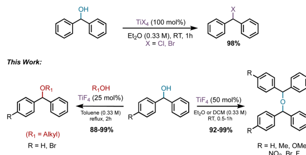
Scheme 1 Reactions of diphenylmethanol with/in the presence of \text{TiX}_4 .
