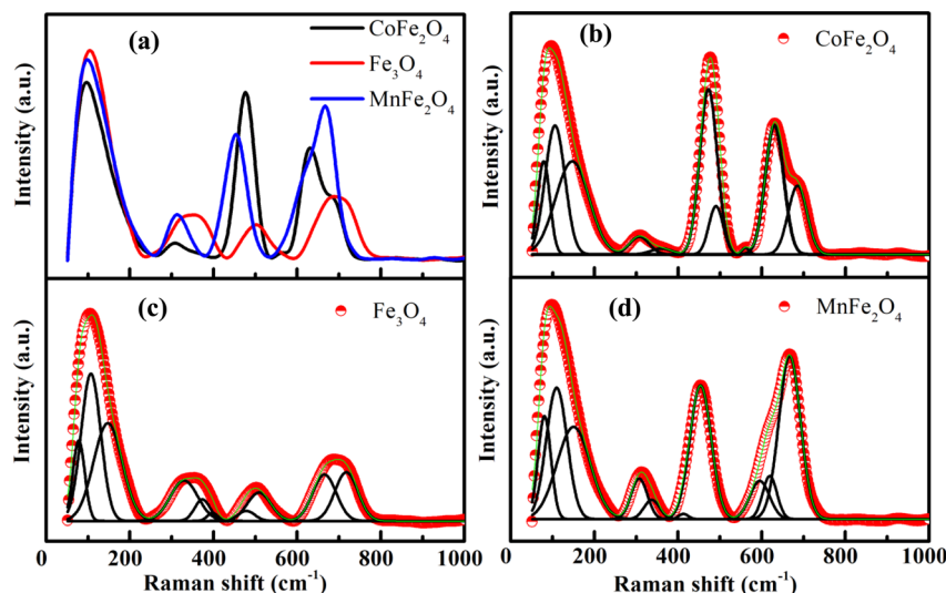
Fig. 6 (a) Experimental Raman spectrum under excitation wavelength of 785 nm and (b–d) Raman active modes fitted with cumulative fit are displayed for \text{MFe}_2\text{O}_4 nanoparticles.
