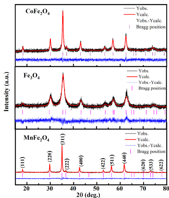
Fig. 2 The Rietveld refinement of XRD patterns for \text{MFe}_2\text{O}_4 nanoparticles (observed – black line, calculated – red line and difference – blue line).
