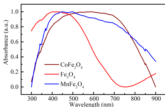
Fig. 7 Room temperature UV-Vis absorbance spectrum of \text{MFe}_2\text{O}_4 nanoparticles.
