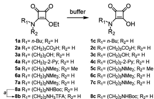
Fig. 1 Structure of the squaramate esters 1a–8b and the corresponding squaric acids 1c–8c obtained from their buffered hydrolysis at 37 °C. a TFA in \text{CH}_2\text{Cl}_2 .
