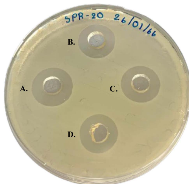
Fig. 3 Preliminary study of the antimicrobial activity of P1-AMP and standard vancomycin demonstrated a clear zone against MRSA isolate 2468 by the agar well diffusion method. The concentration of the standard vancomycin solution (A) was 50 \mu\text{g mL}^{-1} , whereas the concentration of the P1-AMP solutions (B–D) was 118 \mu\text{g mL}^{-1} .
