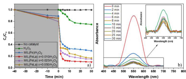
Fig. 9 Cr(vi) photoreduction of various materials over time (a) and absorbance spectra of Cr–DPC solutions after photoreduction over MIL-88B((1 - x)Fe/xLa)-NH 2 (x = 0.010) (b) (initial Cr(vi) concentration: 20 ppm; pH = 6; catalyst dosage: 0.2 g L; H 2 O 2 : 3% (1 mL L -1 ); UV irradiation).
