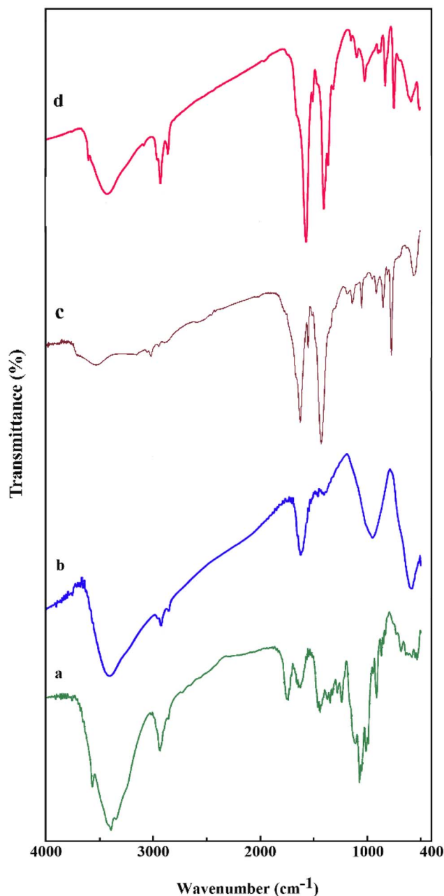
Fig. 2 FT-IR spectra of pectin (a), \text{Fe}_3\text{O}_4 /pectin (b), (Co/Cu)MOF (c) and \text{Fe}_3\text{O}_4 /pectin/(Co/Cu)MOF (d).
