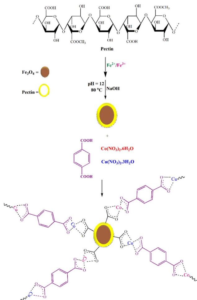
Fig. 1 Preparation of \text{Fe}_3\text{O}_4 /pectin/(Co/Cu)MOF nanocomposite.
