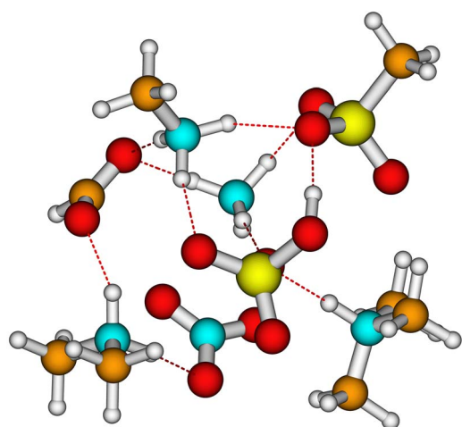
Fig. 1 The (\text{SA})_1(\text{MSA})_1(\text{NA})_1(\text{FA})_1(\text{AM})_1(\text{MA})_1(\text{DMA})_1(\text{TMA})_1 cluster structure lowest in Gibbs free energy at the \omega\text{B97X-D/6-31G++(d,p)} level of theory with the quasi-harmonic approximation (cutoff of 100 \text{ cm}^{-1} ) for the initial sampling. Yellow = sulfur, red = oxygen, cyan = nitrogen, brown = carbon and white = hydrogen.
