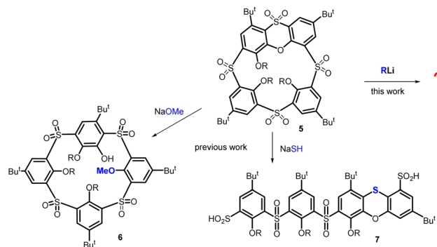
Scheme 2 Cleavage of the phenoxathiin moiety by different nucleophiles.
