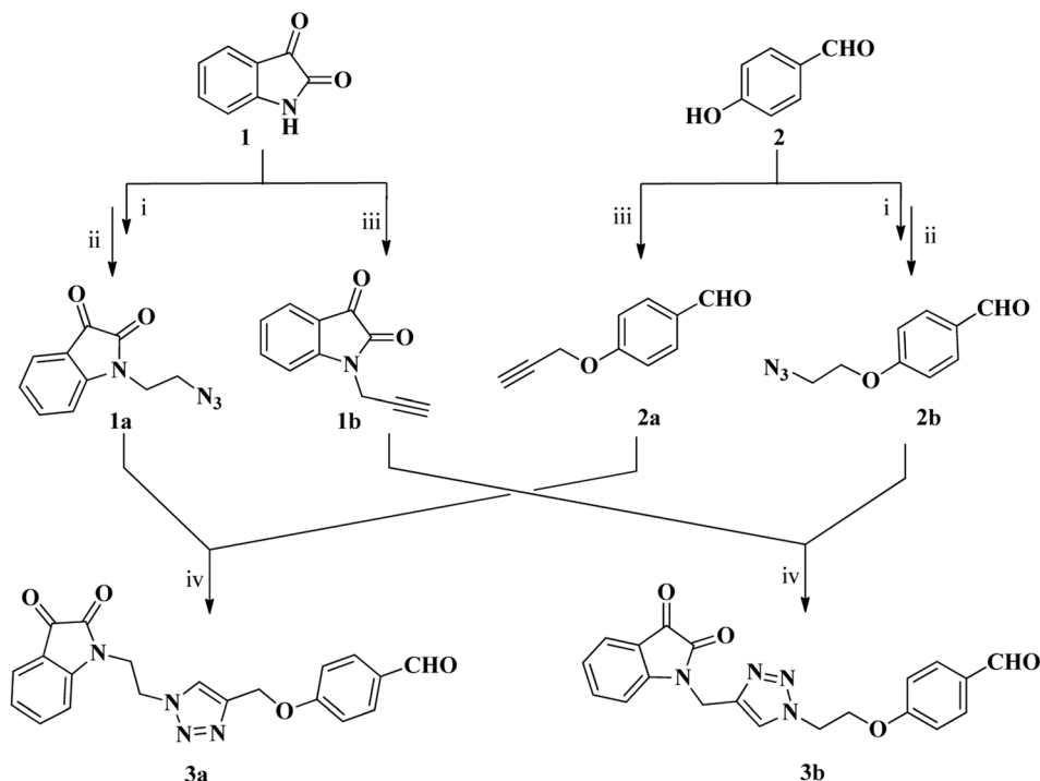
Scheme 1 Synthesis of isatin-triazole hybrids 3a and 3b ; reagents and conditions: (i) dibromoethane (2.1 eq.), DMF, K 2 CO 3 (ii) NaN 3 (1.2 eq.), DMF (iii) propargyl bromide, DMF, K 2 CO 3 (iv) CuSO 4 ·5H 2 O, sodium ascorbate, EtOH : H 2 O (9 : 1), rt.
