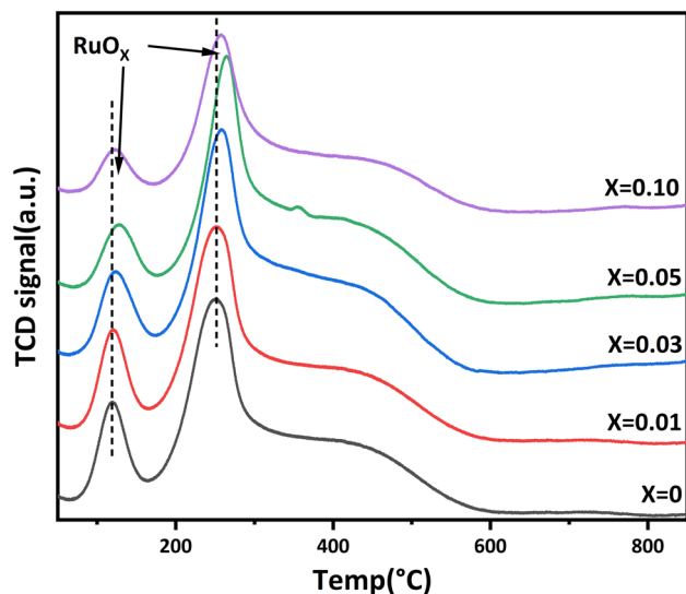
Fig. 9 H_2 -TPR curves of Ru/Ba- Mg_{(1-x)}Zn_xO catalysts.
