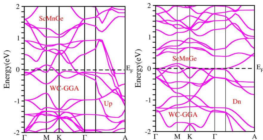
Fig. 6 Illustration of the electronic band structure of ScMnGe alloy using WC-GGA approximation for spin-up and down configuration.
