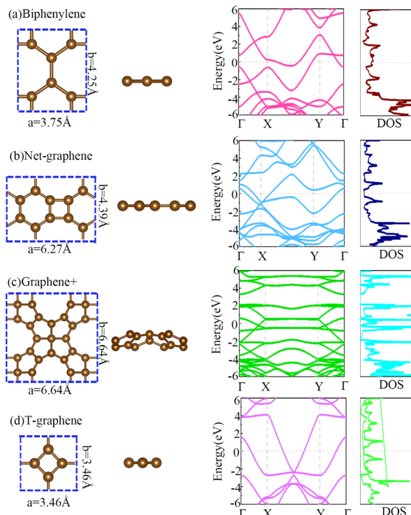
Fig. 1 Unit-cell structure, side view, energy band, and density of states (DOS) of (a) biphenylene, (b) net-graphene, (c) graphene+ and (d) T-graphene. The blue dotted box represents the cells of each structure. Set the zero energy level to the Fermi level, represented by a gray horizontal dotted line.
