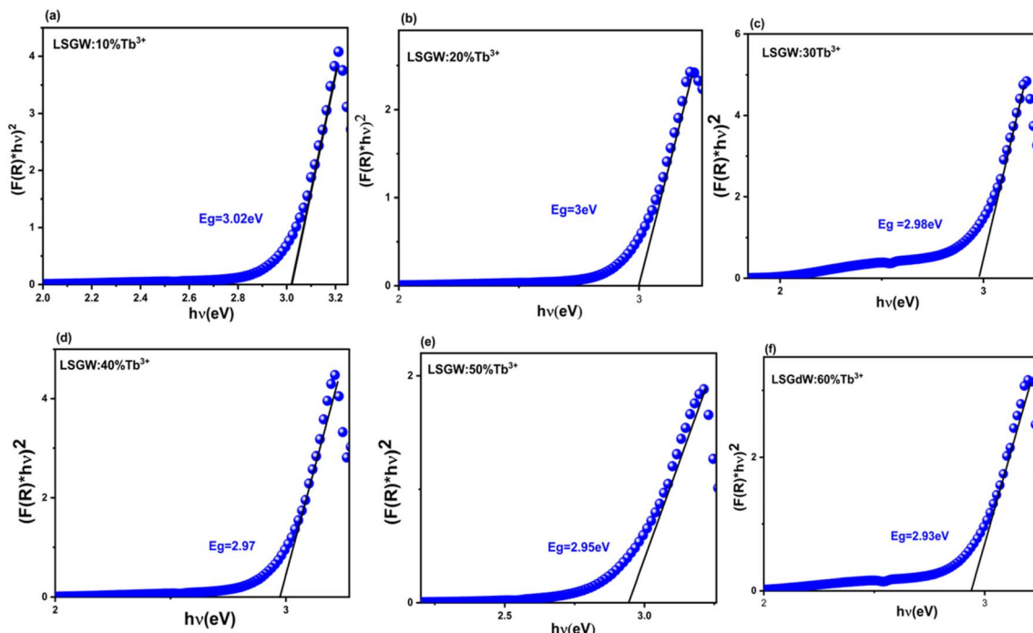
Fig. 4 Plot of [F(R)hv]^2 versus (h\nu) of LSGW doped with (a) 0.1, (b) 0.2, (c) 0.3, (d) 0.4, (e) 0.5 and (f) 0.6 Tb^{3+} , respectively.
