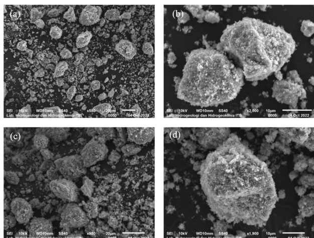
Fig. 4 Structure and morphology samples by SEM (a) and (b) Ti-A and (c) and (d) Ti-B.
