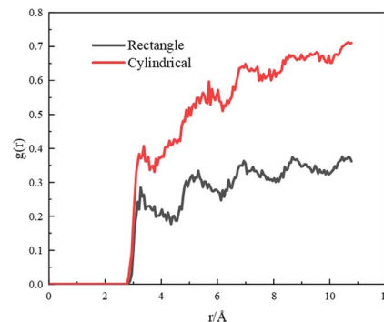
Fig. 9 The radial distribution functions for different surface micromorphology of APG–Cu with a depth \delta of 1.25 nm.
