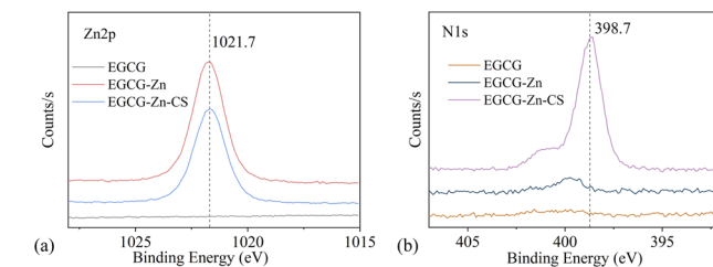
Fig. 4 XPS spectrum of EGCG, EGCG-Zn and EGCG-Zn-CS, high-resolution XPS spectra of Zn 2p (a) and N 1s (b).
