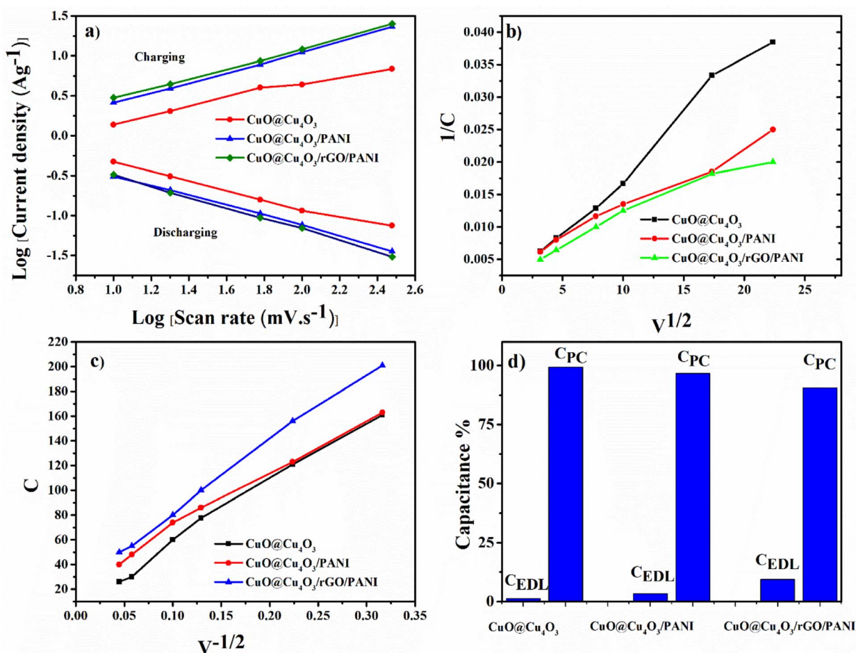
Fig. 6 (a) Linear plot of \log i vs. \log \nu in both charge and discharge processes, (b) plot of 1/C versus \sqrt{\nu} , (c) plot of C versus \nu^{-1/2} , (d) contribution of electric double-layer capacitance and pseudo capacitance for CuO@Cu 4 O 3 , CuO@Cu 4 O 3 /PANI and CuO@Cu 4 O 3 /rGO/PANI.
