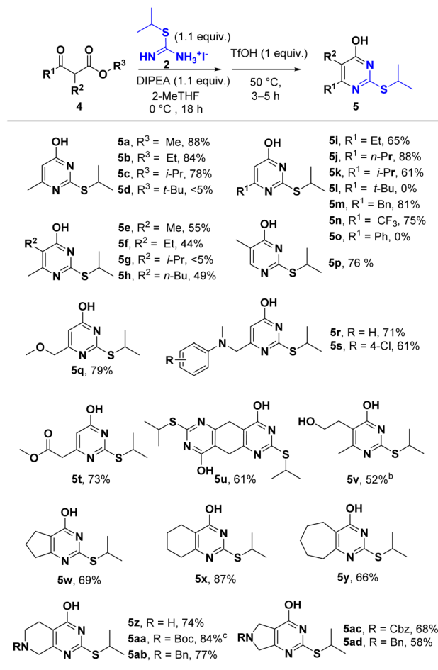
Scheme 3 Substrate Scope of \beta -ketoester a . a Unless otherwise noted, ethyl \beta -ketoester substrate were applied and reactions were conducted as follows: to a solution of S -alkylisothiouronium iodide (1.1 equiv.) and \beta -ketoester (3.0–6.0 mmol, 1.0 equiv.) in 2-MeTHF (0.33 M with respect to \beta -ketoester) at 0 °C was added DIPEA (1.1 equiv.) dropwise. The reaction stirred at 0 °C for 18 hours and then was added with TfOH (1.0 equiv.) dropwise. The reaction was heated to 50 °C in 0.5 h and then stirred for 3–5 hours. b 2-Acetylbutyrolactone was used as the starting material. c deBoc product was obtained.
