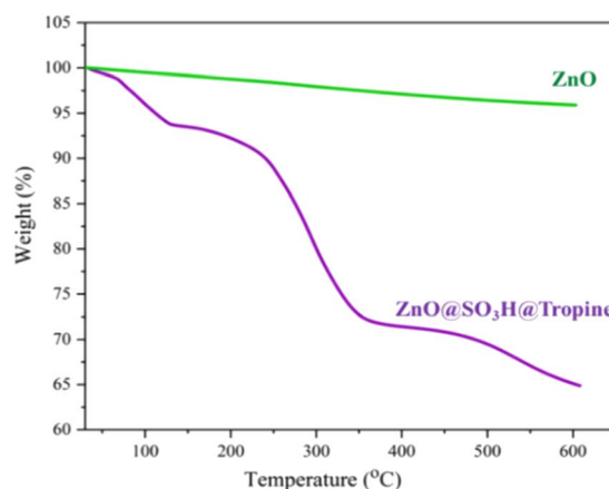
Fig. 3 TGA curve of ZnO and ZnO@SO 3 H@Tropine.
