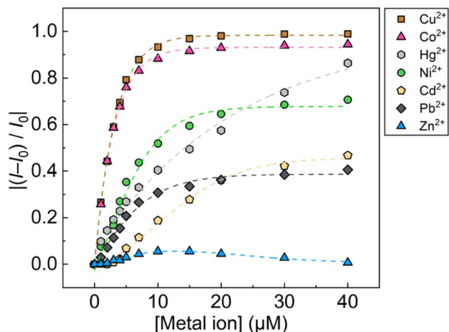
Fig. 3 Fluorescence changes in 1_{\text{poly}} ( 4.0 \times 10^{-5} M per unit) upon the addition of metal ions ( 0.0-4.0 \times 10^{-5} M) in an aqueous MeOH solution (MeOH : water = 3 : 1, v/v) containing MES (12.5 mM) and NaCl (12.5 mM) of pH 5.5 at 25 °C. The terms I_0 and I indicate fluorescent intensity at \lambda_{\text{em}} = 550 nm before and after adding metal ions.
