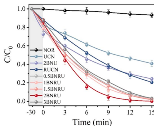
Fig. 18 NOR degradation-based photocatalytic activity. 201
