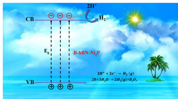
Fig. 24 Water splitting via photocatalytic hydrogen evolution. 274
