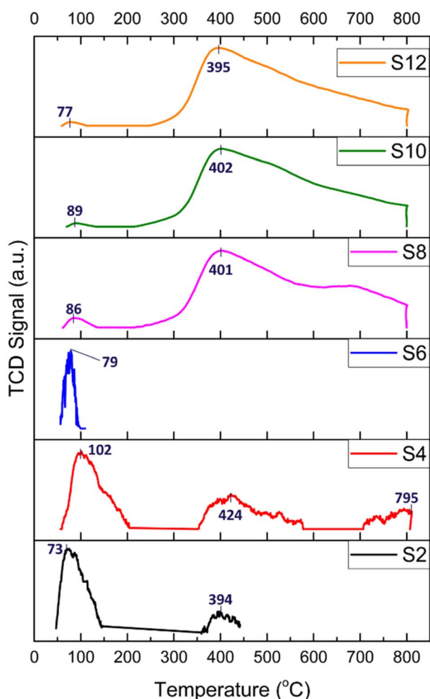
Fig. 6 \text{CO}_2 -TPD profiles of the HNT-supported Ni catalysts; numbers indicate desorption temperatures.
