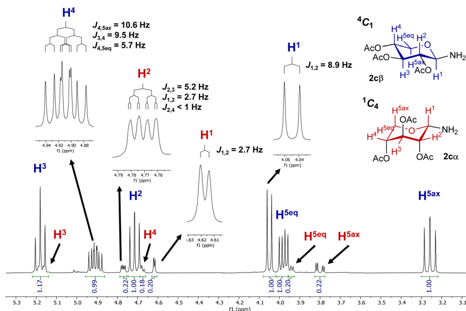
Fig. 1 ^1H NMR spectrum of the mixture of N -glycosyl amines 2cβ and 2cα.
