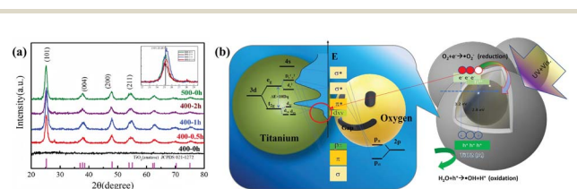
Fig. 4 (a) X-ray diffraction patterns of nanospheres. (b) The mechanism of mobile electron transfer and hole increase under UV-vis illumination. 124
