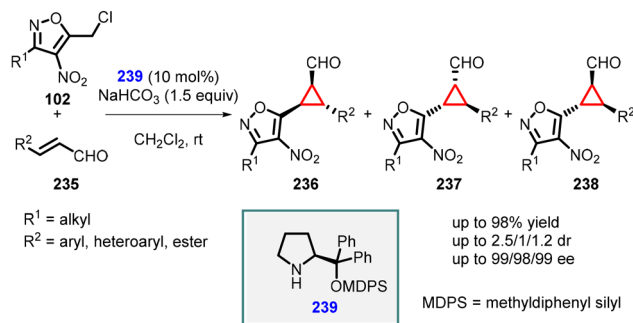
Scheme 53 MIRC cyclopropanation of 5-(chloromethyl)-3-methyl-4-nitrosoxazole and \alpha,\beta -unsaturated aldehydes.
