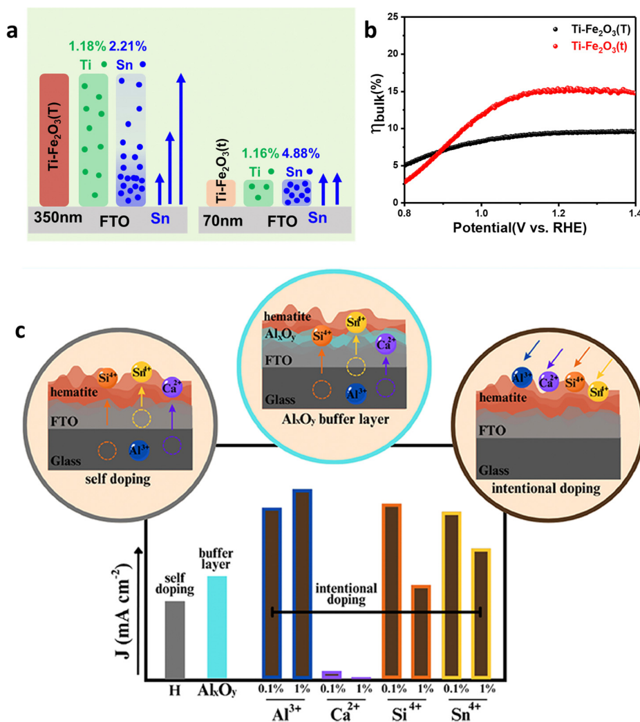
Fig. 9 Intentional and unintentional doping. (a) Distribution of Sn 4+ and Ti 4+ dopants in Ti-Fe 2 O 3 (T) and Ti-Fe 2 O 3 (t) systems. (b) Bulk charge separation efficiency (η bulk ) of Ti-Fe 2 O 3 (T) and Ti-Fe 2 O 3 (t). Reproduced from ref. 94 with permission from Elsevier, copyright 2020. (c) Difference between intentional and unintentional doping. Reprinted with permission from ref. 95, Copyright 2023 American Chemical Society.
