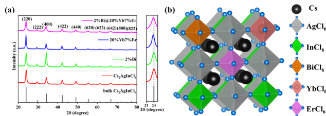
Fig. 1 (a) XRD patterns of Cs 2 AgInCl 6 , Cs 2 AgInCl 6 :2%B i (denoted as 2%B i ), Cs 2 AgInCl 6 :20%Y b , 7%E r (denoted as 20%Y b , 7%E r ) and Cs 2 AgInCl 6 :2%B i @20%Y b , 7%E r (denoted as 2%B i @20%Y b , 7%E r ) NCs (left) and the zoomed-in XRD patterns in the range of 23–24.5° (right); (b) schematic structure illustrating the unit cells of Bi 3+ -doped Cs 2 AgInCl 6 and Yb 3+ , Er 3+ co-doped Cs 2 AgInCl 6 for brevity.
