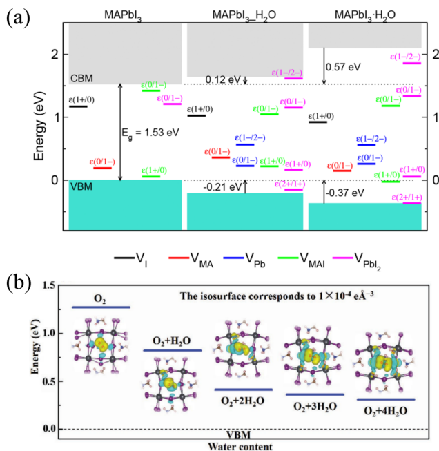
Fig. 5 (a) Band alignment and thermodynamic transition levels in MAPbI 3 , water-intercalated MAPbI 3 ·H 2 O, and monohydrate MAPbI 3 ·H 2 O, where deep-lying Pb 5d levels are used as a reference for the VBM and CBM of each phase. Reproduced with permission. 56 Copyright 2018, American Chemical Society. (b) Minimum energy level of \pi^*2p of O 2 adsorbed at the interstitial space on a PbI 2 -terminated surface as a function of water content. Reproduced with permission. 59 Copyright 2019, John Wiley and Sons.
