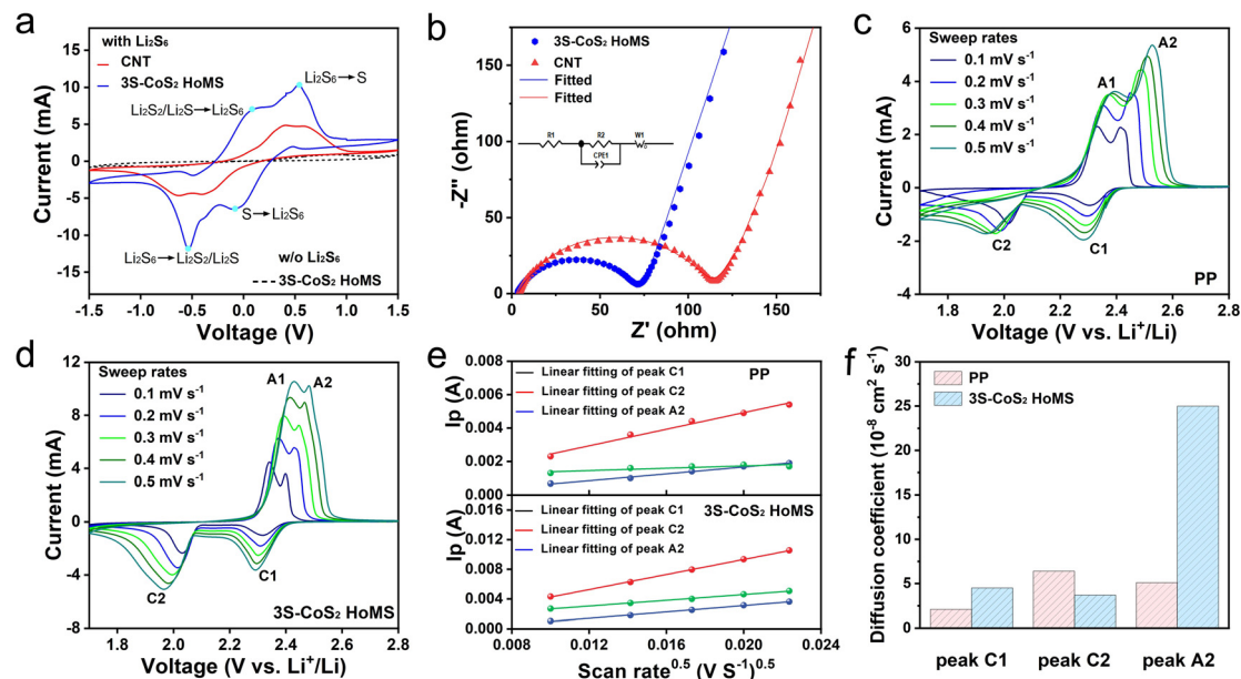
Fig. 3 Comparison of the kinetic behaviors of batteries using different separators. (a) CV curves at a scan rate of 5 mV s -1 and (b) EIS spectra of the \text{Li}_2\text{S}_6 symmetric battery, employing CNT and 3S-CoS 2 HoMS as the identical electrodes. (c-e) CV curves of the Li-S cells with the PP separator (c) and 3S-CoS 2 HoMS-coated separator (d) at different scan rates from 0.1 to 0.5 mV s -1 , and (e) corresponding linear fits of the peak currents. (f) Comparison of lithium ion diffusion coefficients for the Li-S batteries.
