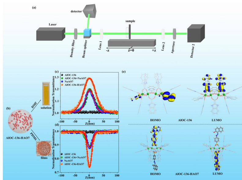
Fig. 4 NLO investigation. (a) Schematic representation of the Z-scan setup. (b) Sample preparation methods in different media. The figure shows AIOIC-136-HAO7 as an example. (c) OA Z-scan curves of samples dispersed in DMF solution with nanosecond laser duration excitation (input energy: 100 \mu\text{J} ). (d) OA Z-scan curves of samples dispersed in PDMS films with nanosecond laser duration excitation (input energy: 100 \mu\text{J} ). (e) The frontier molecular orbital theoretical view of the HOMO and LUMO states of AIOIC-136 and AIOIC-136-HAO7 .
