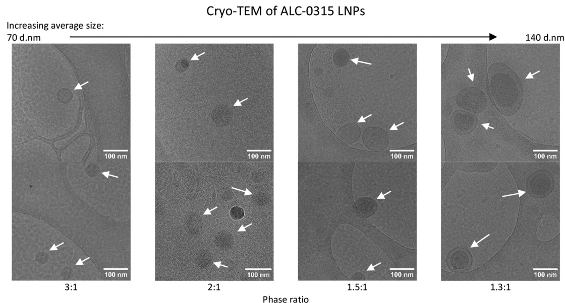
Fig. 4 Cryogenic transmission electron microscopy of LNPs with ALC-0315 as the ionisable lipid, manufactured at four different aqueous:lipid phase ratios. There are two images at 30 000 \times magnification for each manufacturing phase ratio, and LNPs are shown by white arrows. The LNPs were manufactured with an N/P ratio of 6 from 5 mg mL -1 lipid stock. pH 7.4 PBS was used as the exchange buffer, and they were maintained in this buffer at manufacturing concentrations when cryogenically frozen in liquid ethane and imaged in liquid nitrogen using a Jeol JEM-F-200 microscope at 200 kV.
