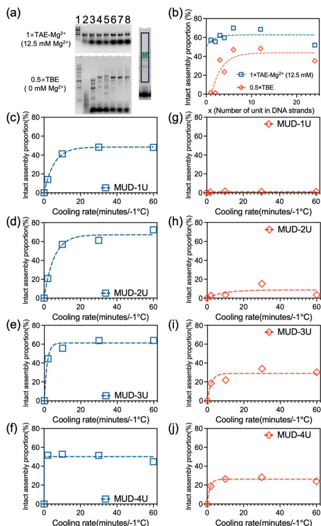
Fig. 4 (a) Images of a series of MUD- x U samples under agarose-gel electrophoresis with 1x TAE-Mg 2+ (Mg 2+ = 12.5 mM) buffer (upper-left panel) and 0.5x TBE buffer (Mg 2+ = 0 mM) (lower-left panel). All MUD- x U samples were assembled with 20 mM Mg 2+ in the buffer. Lanes 1, 2, 3, 4, 5, 6, 7, and 8: double-stranded DNA ladder (GeneRuler Express DNA Ladder, Thermo Fisher Scientific), MUD-1U, MUD-2U, MUD-3U, MUD-4U, MUD-6U, MUD-12U, and MUD-24U, respectively. Right panel: areas of intact assembly and total assembly products used for calculating the proportion of intact assemblies were marked by the green mask and black box, respectively. (b) Analyses of intact proportions of a series of MUD- x U samples under agarose-gel electrophoresis with 1x TAE-Mg 2+ buffer (Mg 2+ = 12.5 mM, marked by blue boxes) and 0.5x TBE buffer (Mg 2+ = 0 mM, marked by red diamonds). The intact assembly proportions of (c and g) MUD-1U, (d and h) MUD-2U, (e and i) MUD-3U, and (f and j) MUD-4U with different cooling rates under agarose-gel electrophoresis containing 12.5 mM Mg 2+ (marked in blue boxes) and 0 mM Mg 2+ (marked in red diamonds). The one-phase decay-fitting curves corresponding to the sample data in the same color are presented in (b)–(j).
