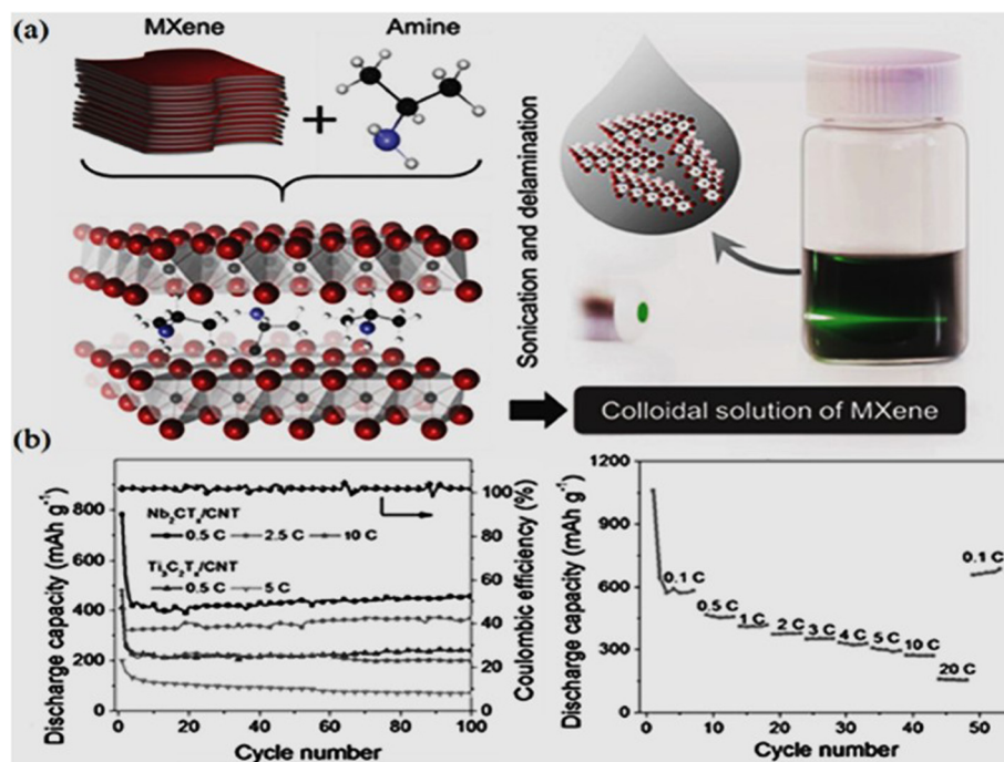
Fig. 12 (a) Schematic representation of the delamination process of \text{Nb}_2\text{CT}_x (MXene); (b) cycling stability and rate performance of \text{Nb}_2\text{CT}_x/\text{CNT} paper electrodes. Reprinted with permission from ref. 222. Copyright John Wiley and Sons.
