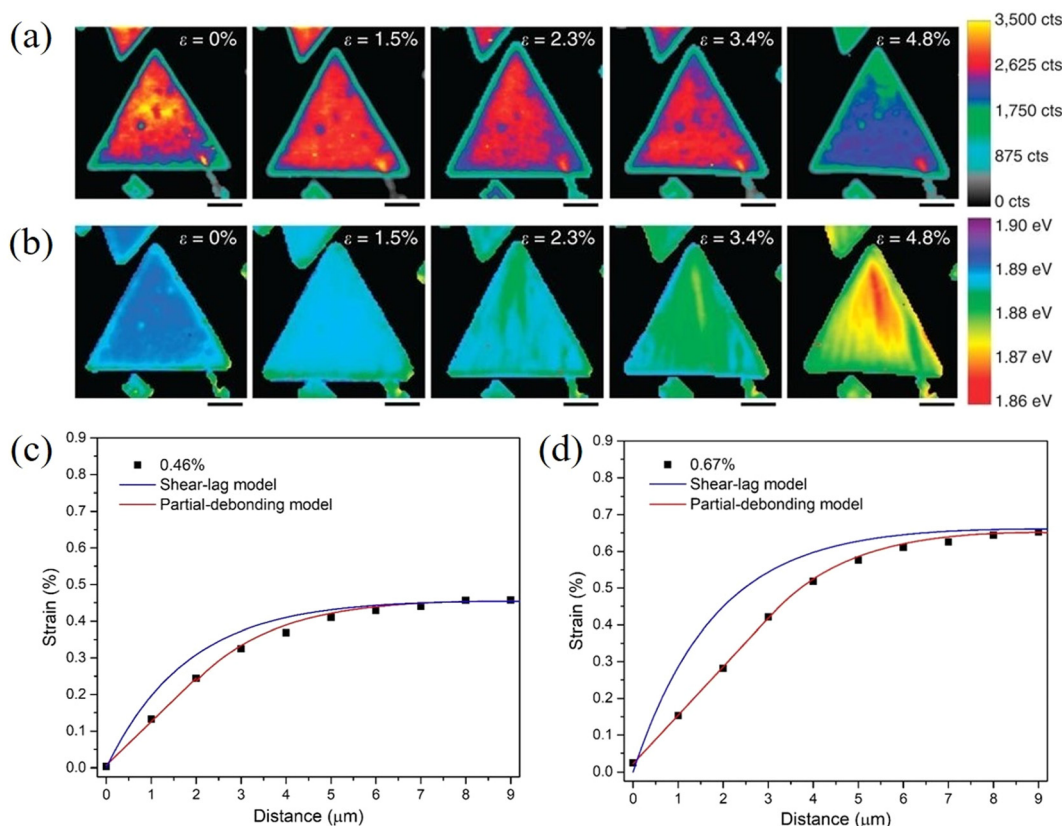
Fig. 8 PL A exciton (a) intensity and (b) peak mapping of MoS 2 with applied strain increasing from 0 to 4.8%. (Scale bar, 4 \mu m). Reproduced with permission from ref. 114. Copyright 2014 Nature Publishing Group. Strain distribution in monolayer MoS 2 at (c) 0.46% and (d) 0.67% strain. Both shear-lag model and partial-debonding model were used to fit the experimental results. Reproduced with permission from ref. 115. Copyright 2023 Elsevier.
