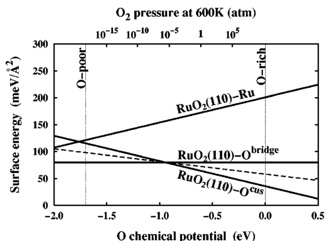
Fig. 2 Surface free energies, \gamma(T, p_{O_2}) , for three possible RuO_2(110) terminations calculated over the allowed range of oxygen chemical potential, \mu_O(T, p_{O_2}) , as indicated by the vertical dashed lines. The sloped dashed line depicts the surface free energy of a RuO_2(110)-O^{\text{cus}} termination with only every second O^{\text{cus}} site occupied. This figure has been reproduced from ref. 9 with permission from the American Physical Society, copyright 2001.
