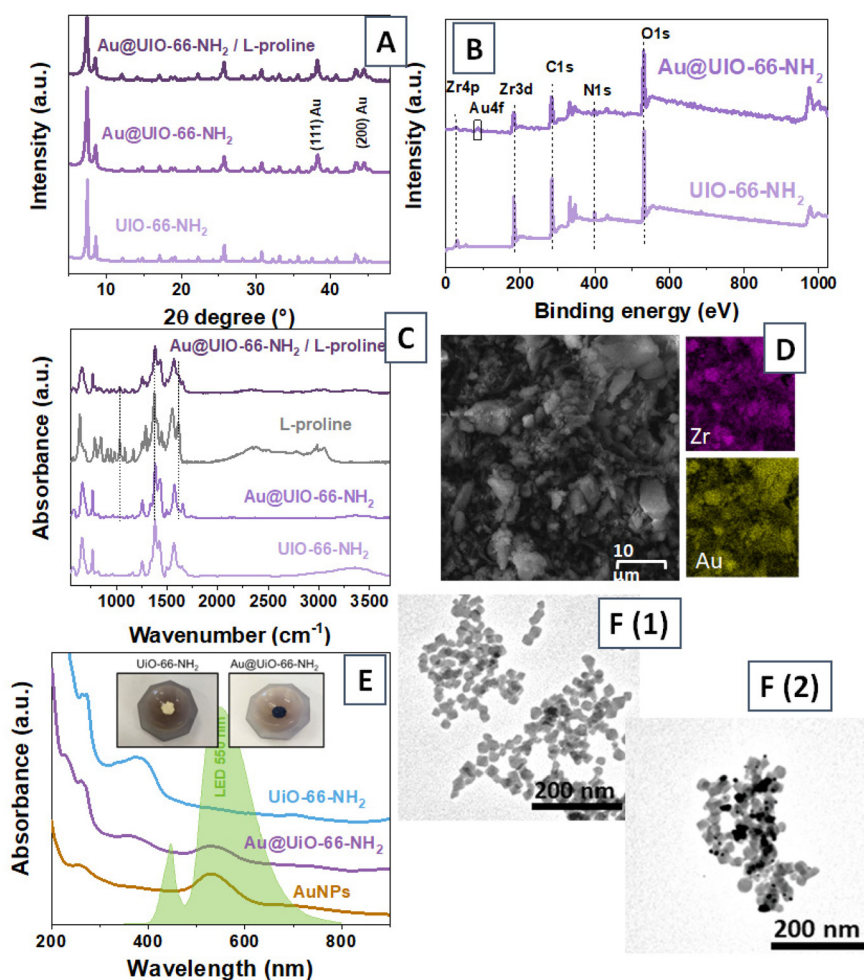
Fig. 2 Characterization of the catalyst structure: (A) XRD patterns of separately prepared UiO-66-NH 2 powder and Au@UiO-66-NH 2 powders before and after proline entrapping; (B) XPS survey spectra of UiO-66-NH 2 and Au@UiO-66-NH 2 powders; (C) FTIR absorption spectra of separately prepared UiO-66-NH 2 , proline and Au@UiO-66-NH 2 powders before and after proline entrapping; (D) SEM-EDX characterization of Au@UiO-66-NH 2 (morphology and elemental composition); (E) UV-Vis spectra of Au@UiO-66-NH 2 dispersion and separately prepared AuNPs or UiO-66-NH 2 dispersions (the LED emission spectrum is also presented, the insert shows the photos of UiO-66-NH 2 and Au@UiO-66-NH 2 powders); (F) TEM images of UiO-66-NH 2 (F1) and Au@UiO-66-NH 2 (F2) samples.
