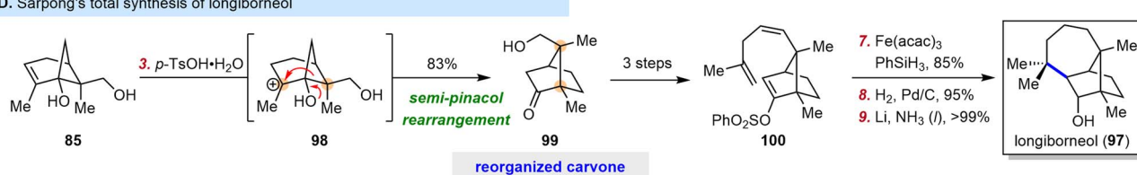
Scheme 11 Sarpong's syntheses of phomactins, xishacorene B and longiborneol.
